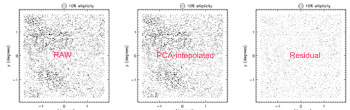
Fig. 7. Ellipticity distribution of the simulated LSST PSFs (left). The middle panel shows the ellipticity distribution of the PCA-interpolated PSFs. Comparison of these two plots along with the residual plot (right) illustrates that our PCA interpolation closely approximates the PSF variation in the LSST field.
